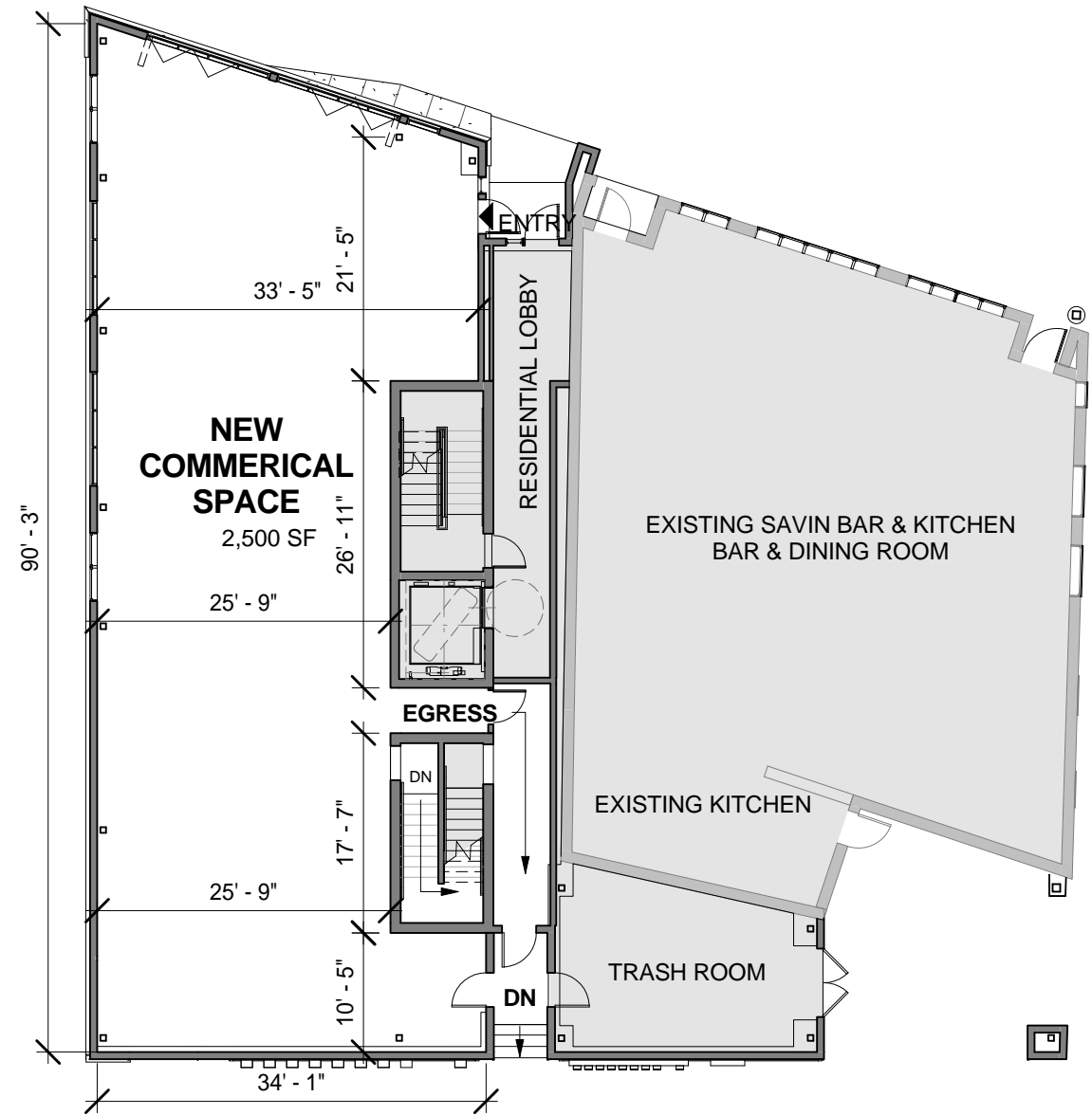
1 FIRST LEVEL 1/16" = 1'-0"
