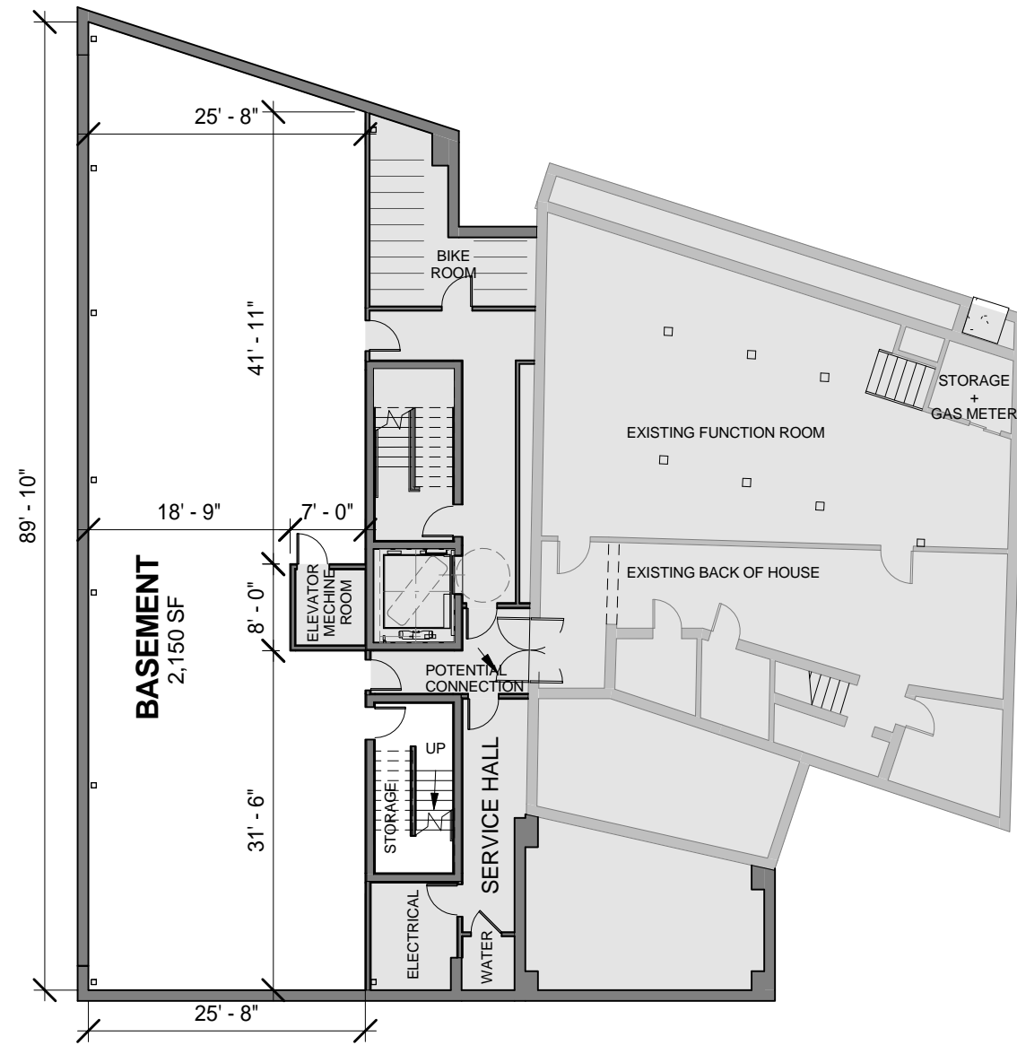
0 BASEMENT LEVEL 1/16" = 1'-0"
