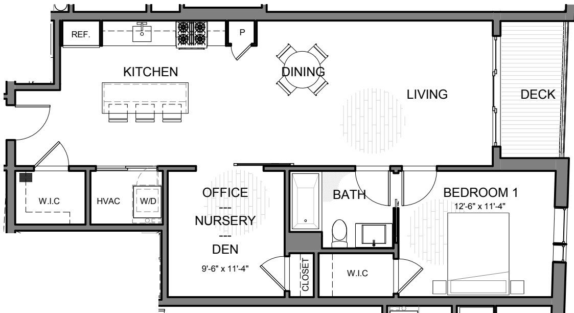
UNIT- 203+303 1+ BEDROOM 880 GSF
